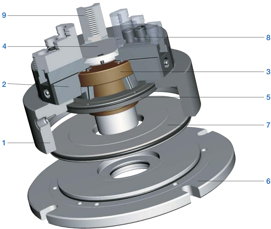
Stationary power chuck SSP
