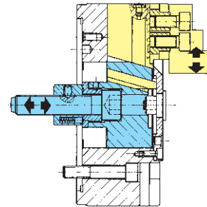
Design principle wedge system
