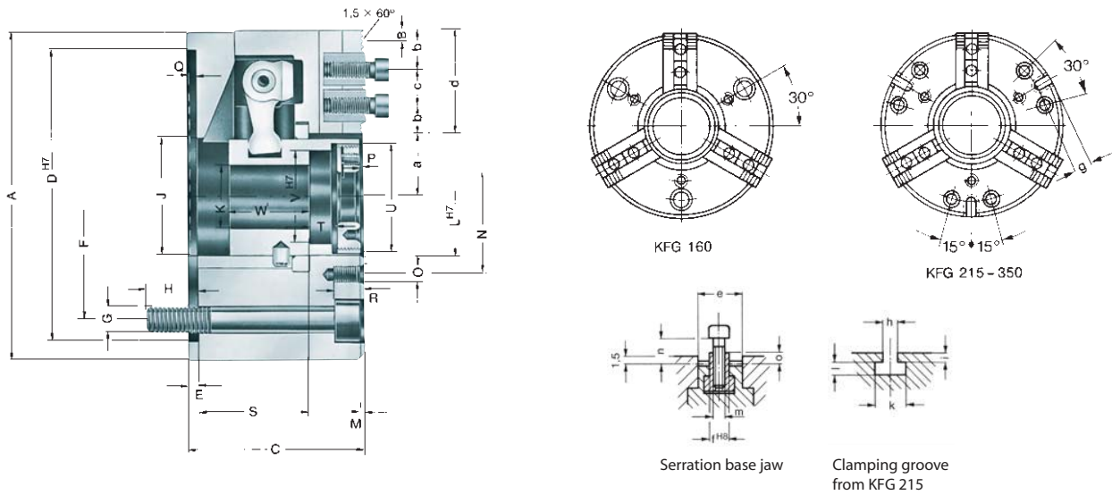
C 15 3-jaw angle lever power chucks KFG, large jaw movement, with serration 60°, cylindrical centre mount
